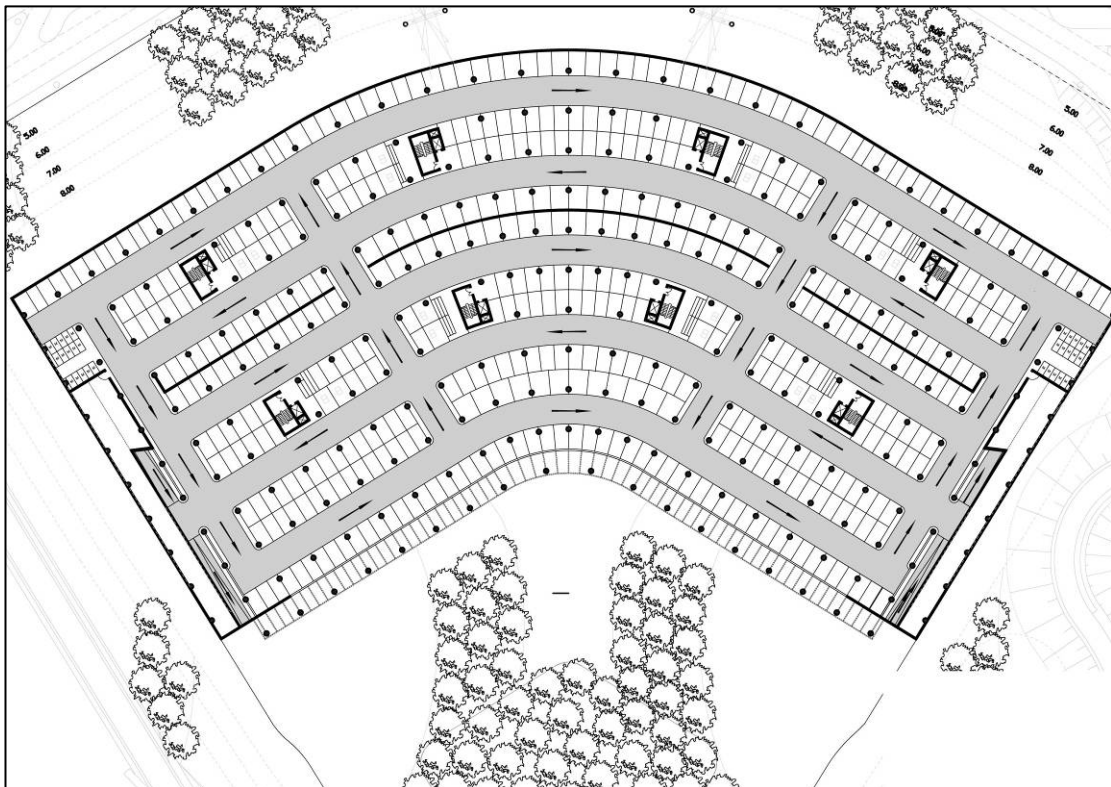
Parking Facility – Third Level
