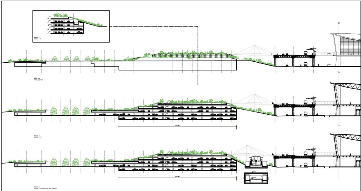
Parking Facility - Cross-Sections
